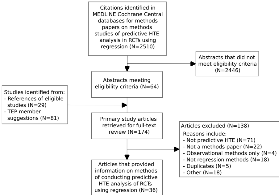
Figure 2.1: Study flow chart.
