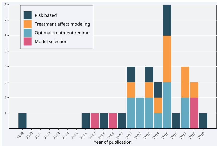
Figure 2.2: Results of the review.
