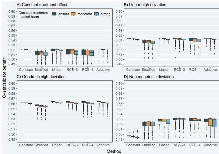
Figure 4.4: Discrimination for benefit of the considered methods across 500 replications calculated in simulated samples of size 4,250 using the c -statistic for benefit. The c -statistic for benefit represents the probability that from two randomly chosen matched patient pairs with unequal observed benefit, the pair with greater observed benefit also has a higher predicted benefit. True prediction c -statistic of 0.75.
