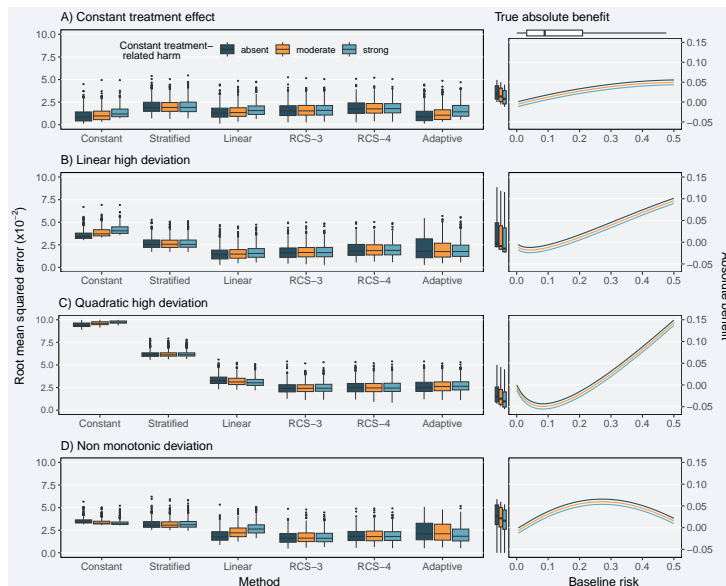
Figure 4.3: RMSE of the considered methods across 500 replications calculated in simulated samples 4,250. True prediction c-statistic of 0.85. RMSE was calculated on a super-population of size 500,000
