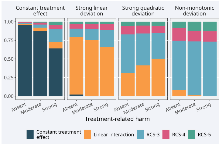
Figure B.2: Model selection frequencies of the adaptive approach based on Akaike’s Information Criterion across 500 replications. Sample size is 17,000.
