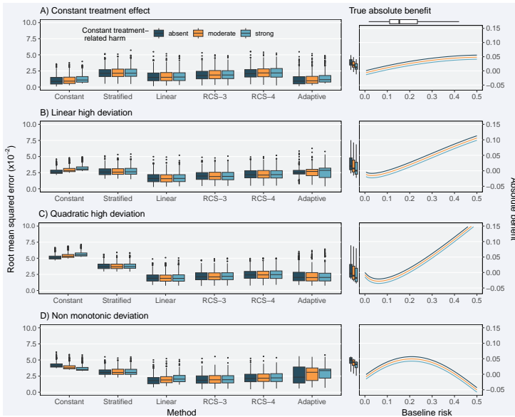
Figure B.11: RMSE of the sensitivity analyses assuming correlated baseline covariates. All considered methods were derived using simulated samples of size 4,250 and true prediction c-statistic of 0.75.
