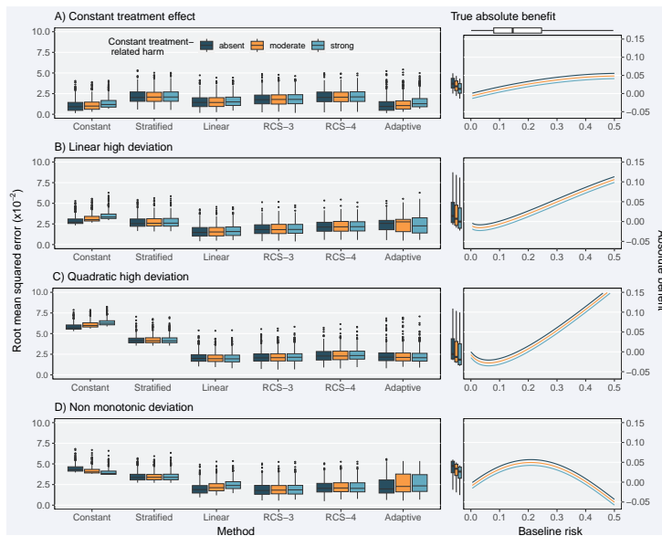
Figure 4.1: RMSE of the considered methods across 500 replications was calculated from a simulated super-population of size 500,000. The scenario with true constant relative treatment effect (panel A) had a true prediction c-statistic of 0.75 and sample size of 4250. The RMSE is also presented for strong linear (panel B), strong quadratic (panel C), and non-monotonic (panel D) deviations from constant relative treatment effects. Panels on the right side present the true relations between baseline risk (x-axis) and absolute treatment benefit (y-axis). The 2.5, 25, 50, 75, and 97.5 percentiles of the risk distribution are expressed by the boxplot on the top. The 2.5, 25, 50, 75, and 97.5 percentiles of the true benefit distributions are expressed by the boxplots on the side of the right-hand side panel.
