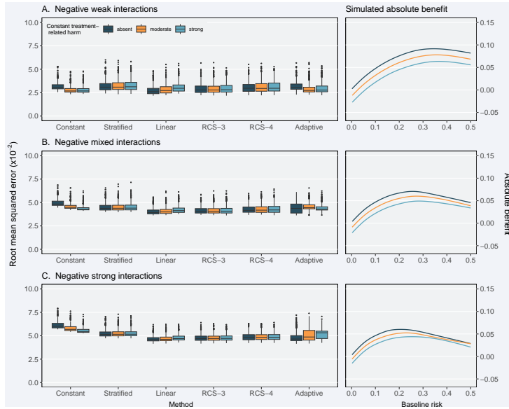
Figure B.9: RMSE of the considered methods across 500 replications calculated in a simulated sample of size 500,000 where treatment-covariate interactions all favoring the control were considered.
